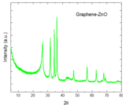
*X-Ray diffraction
