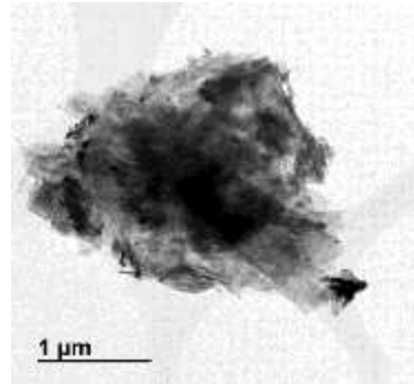
*TEM Image
