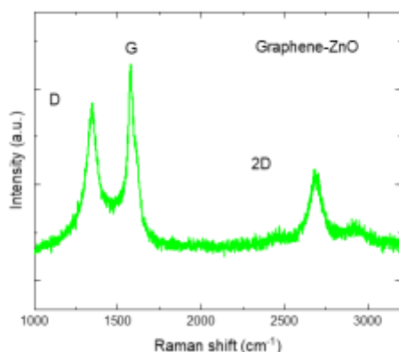
*Raman Spectroscopy
